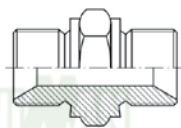
MACHÓN BSP 60° - BSP 60° RC6018
